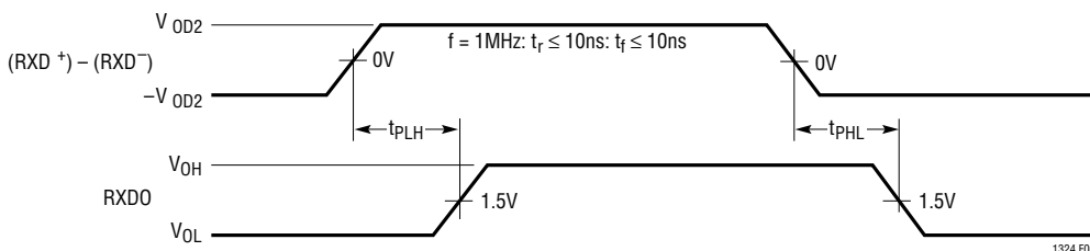
Figure 6. Differential Receiver
